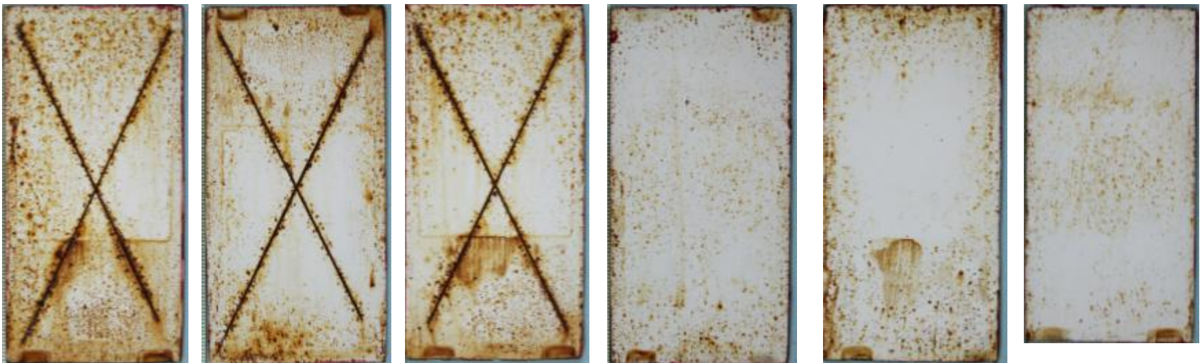
Figure 2. Super Therm coupons' images after six weeks of exposure
